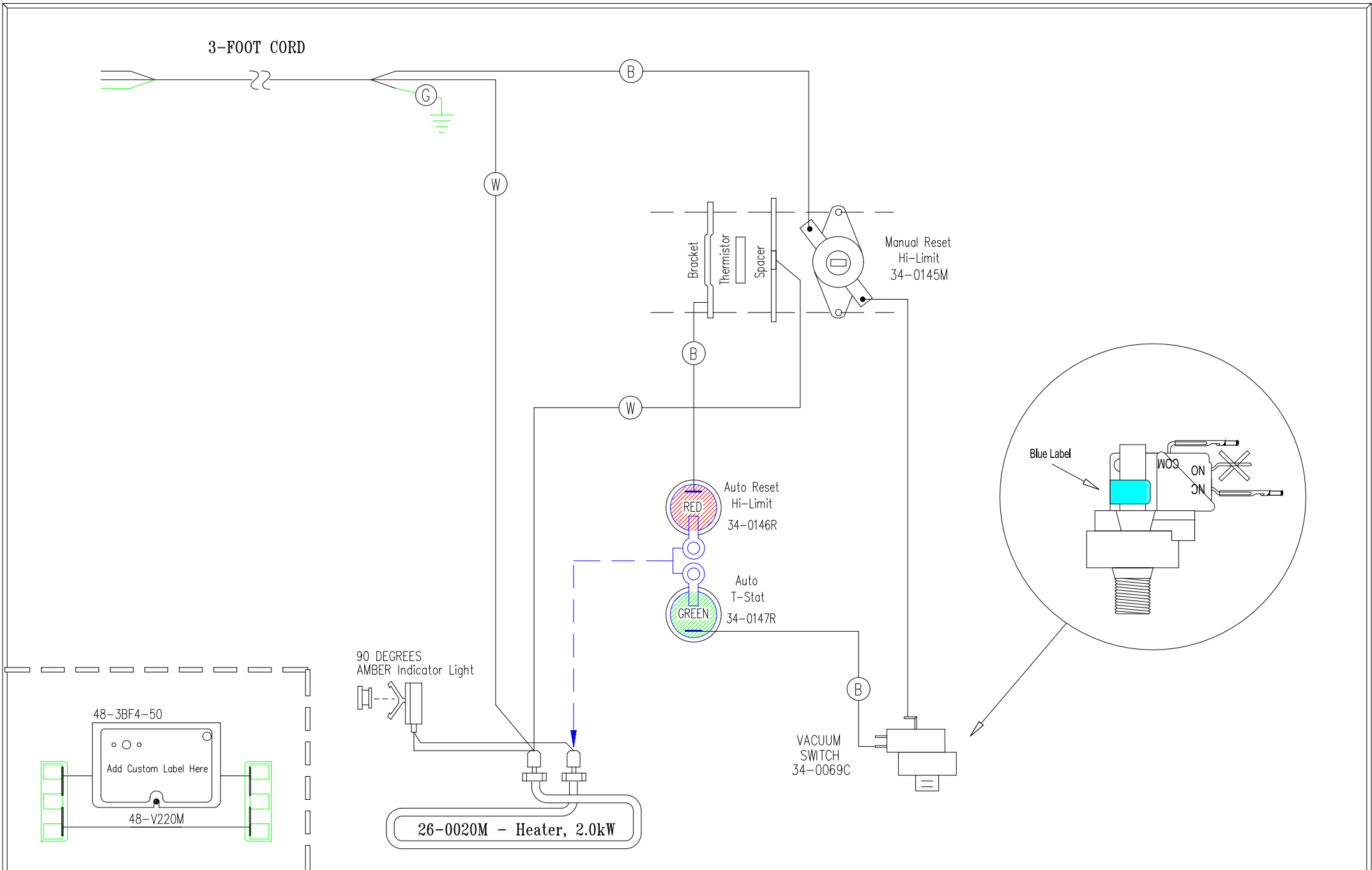
Wiring Diagram, Bath, Depicting New Solderless Wiring
